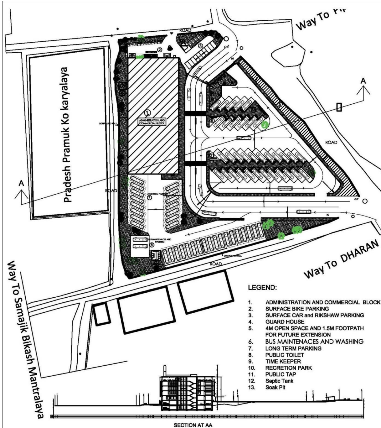
Figure: Terminal Building Plan with Bus Park
